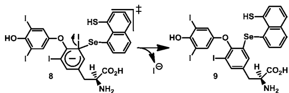
Scheme 3. Possible Mechanism for the Deiodination of T4 by Compound 2
